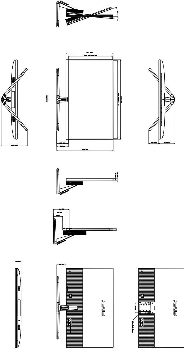
ASUS VU279CFE Outline Dimension *Unit: mm(1inch)
